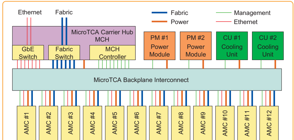
Figure 2. Typical 12-slot MicroTCA Architecture
