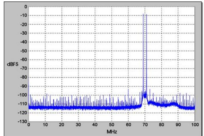
Two-Tone SFDR
