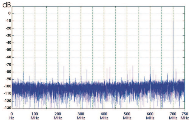
Two-Tone SFDR
