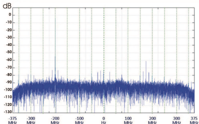
DDC Performance
