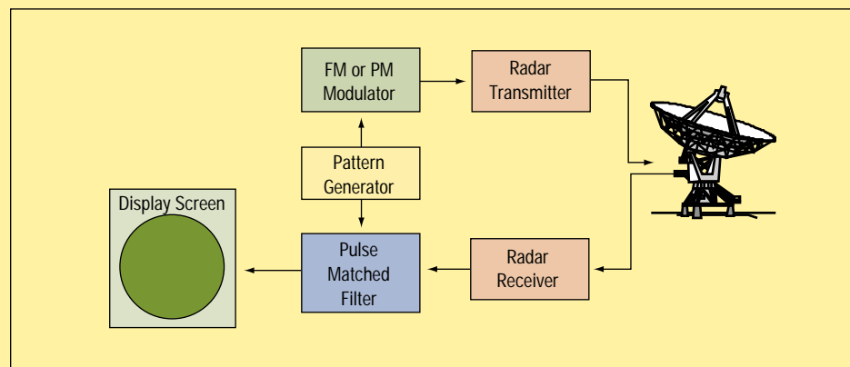
Pulse Compression Radar
