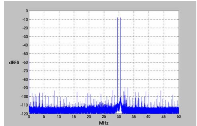
Two-Tone SFDR
