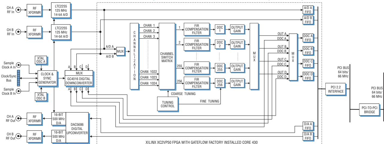
Model 7241-430 and 7341-430 Block Diagram Model 7241-430D doubles all resources except the PCI Bridge
