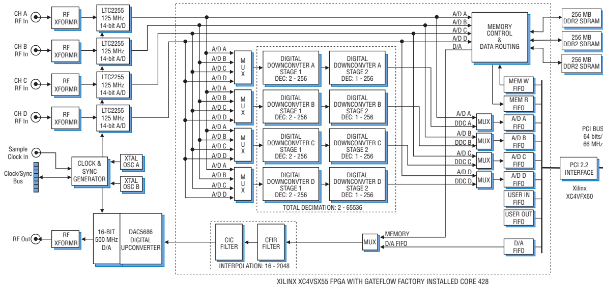
XILINX XC4VXS55 FPGA WITH GATEFLOW FACTORY INSTALLED CORE 428
