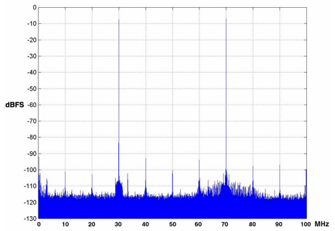
Two-Tone SFDR
